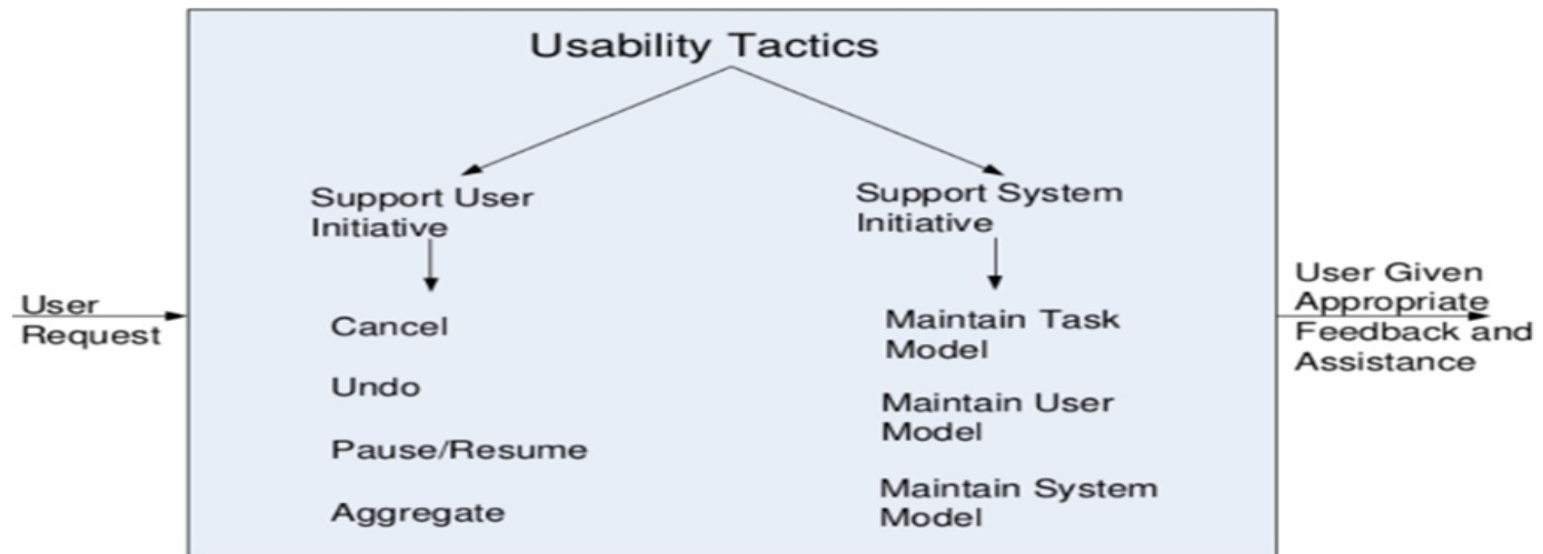
FIGURE 11.2 The goal of runtime usability tactics
